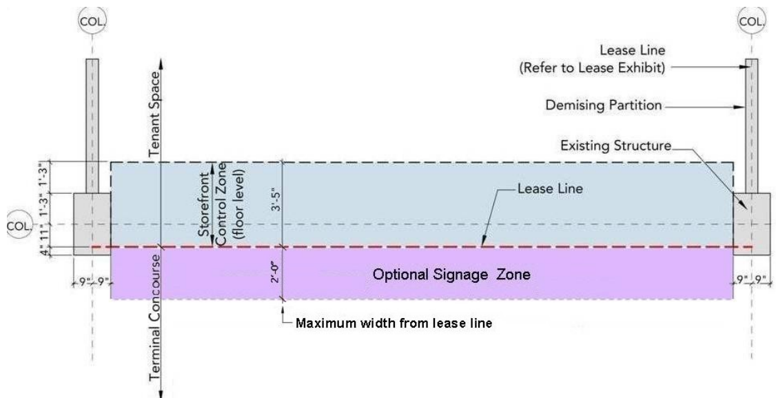
Figure 2.4 – Plan/Optional Signage Location
